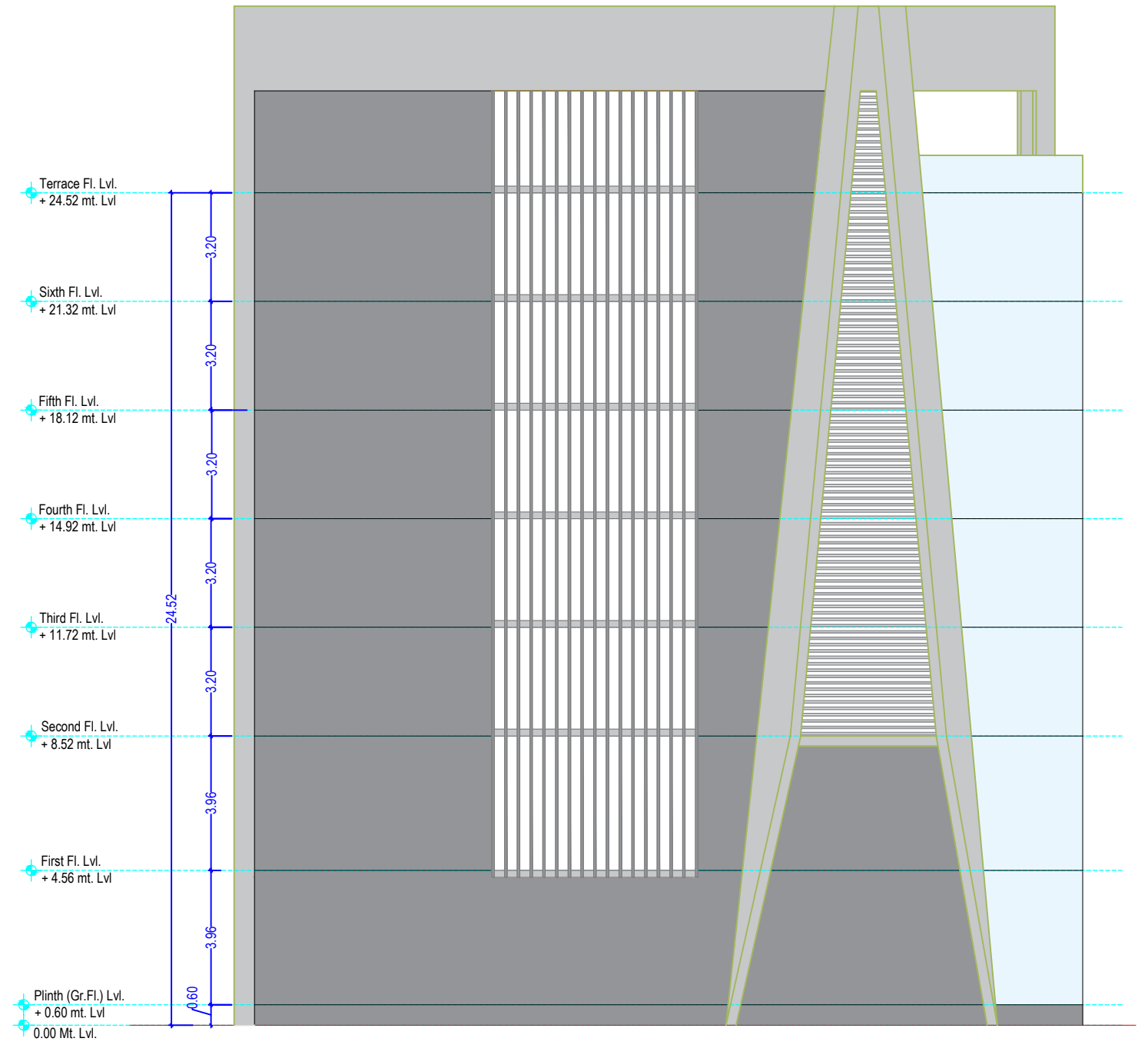
NORTH ELEVATION
