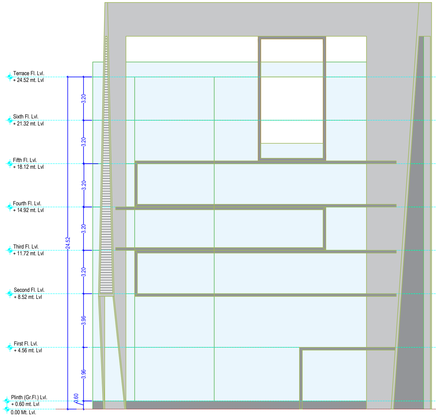
SOUTH ELEVATION
