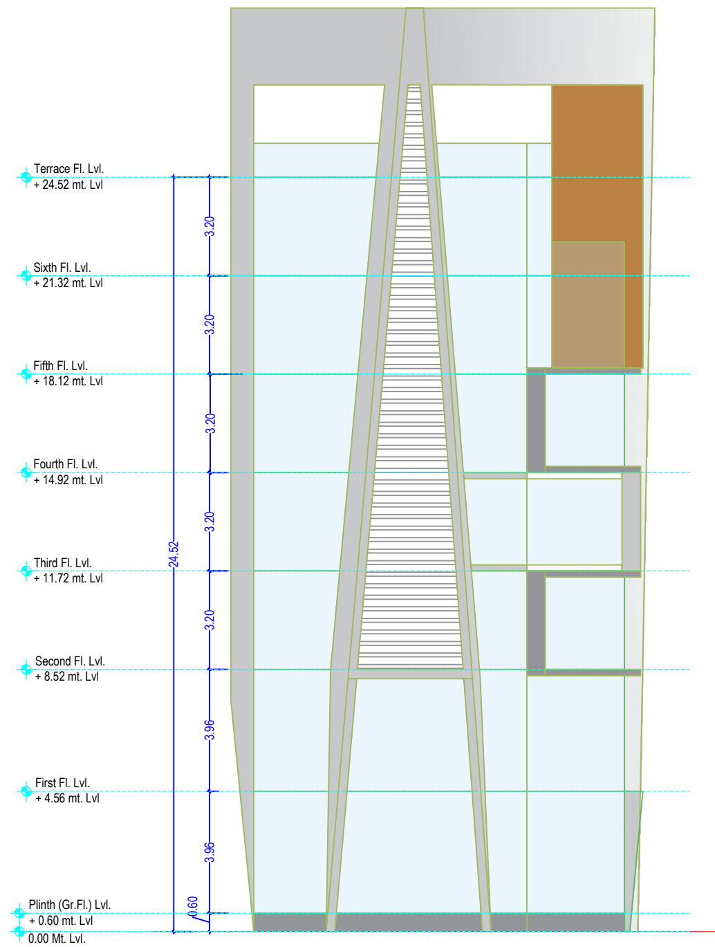
WEST ELEVATION
