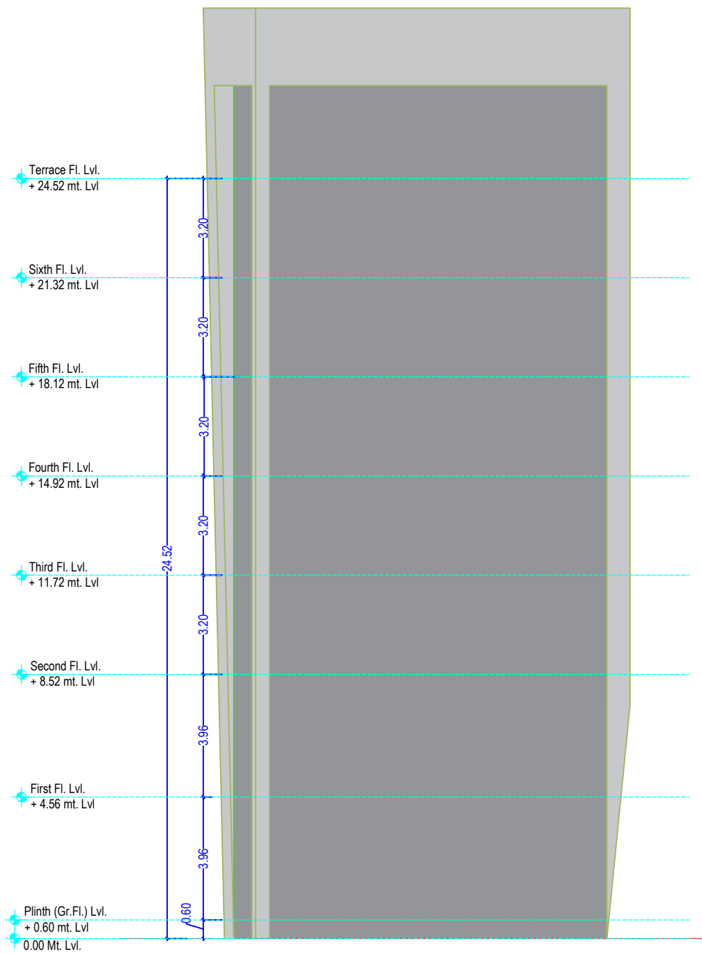
EAST ELEVATION
