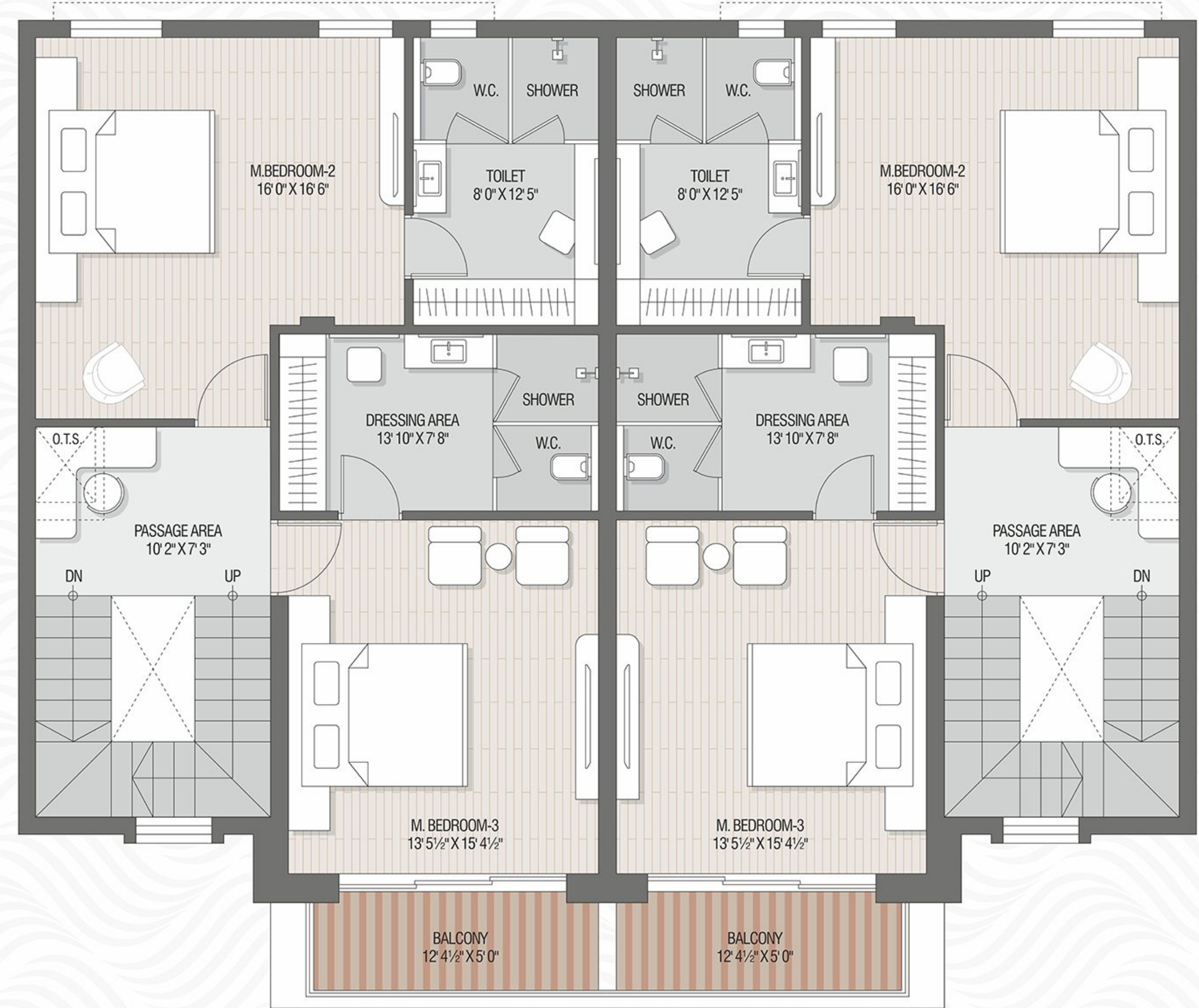
3 BHK | TYPE B 144 SQ.YARD | 25' 1/2" X 51' 7" | FIRST FLOOR PLAN
