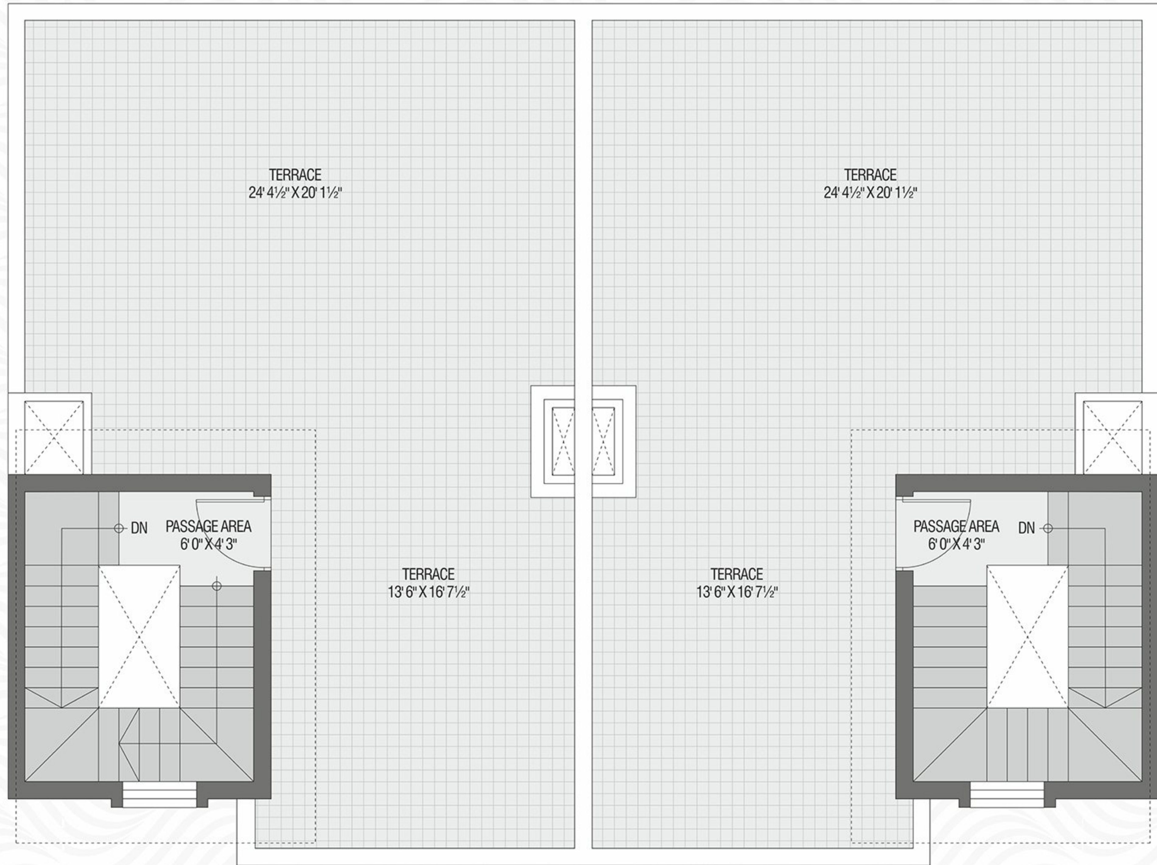
3 BHK | TYPE B 144 SQ.YARD | 25' 1/2" X 51' 7" | TERRACE FLOOR PLAN
