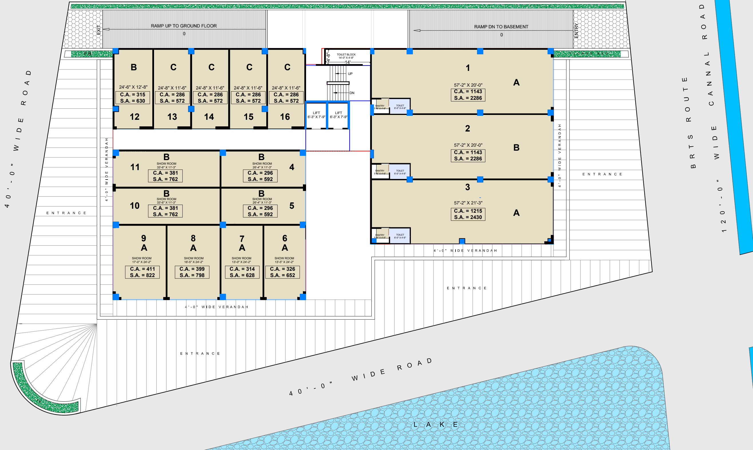
GROUND FLOOR PLAN (16'-0" HT)
